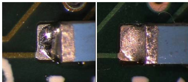
Figure 13: Visual inspection difference between SnPb solder joint (L) and SAC solder joint (R)
