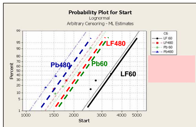
Figure 6: LF Temp cycle performance in long dwell time testing
