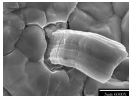
Figure 8: Sn whiskers
