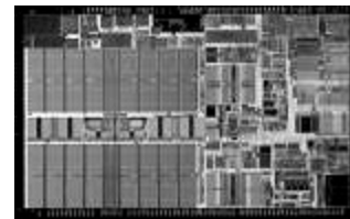
Figure 6: Pentium® III die on 0.13μm process
