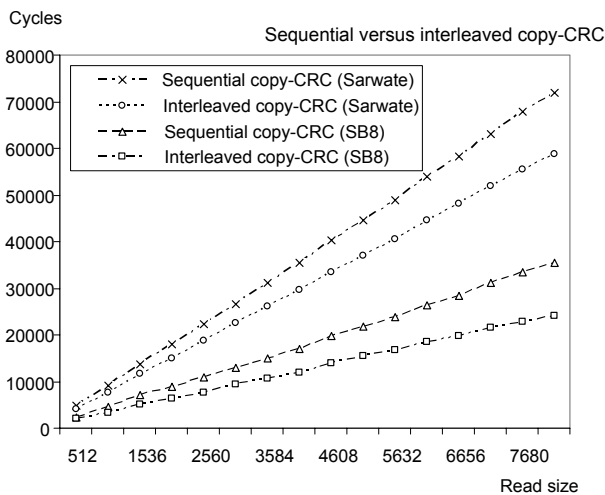
Figure 15: Interleaved Copy-CRC cost
