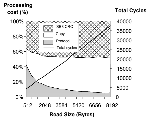
Figure 14: Data-in PDU processing cost (with SB8 CRC)
