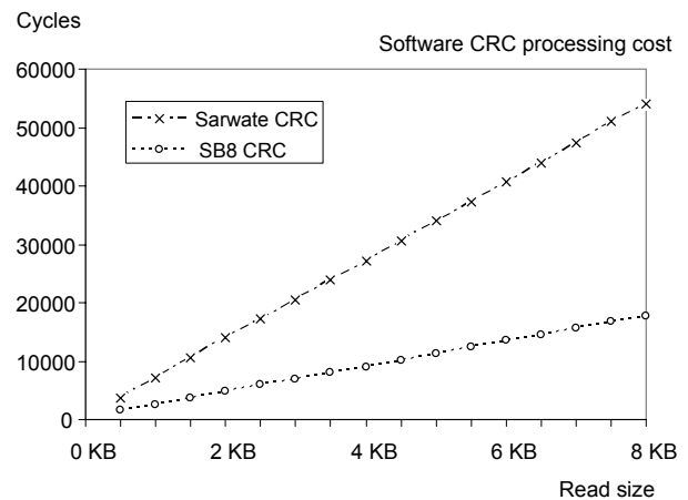
Figure 13: SB8 CRC versus Sarwate CRC
