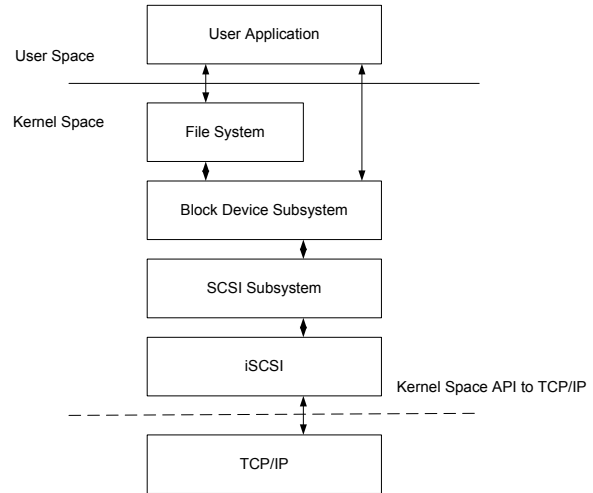
Figure 1: Typical initiator protocol stack
