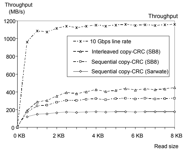
Figure 16: Projected software Read throughput
