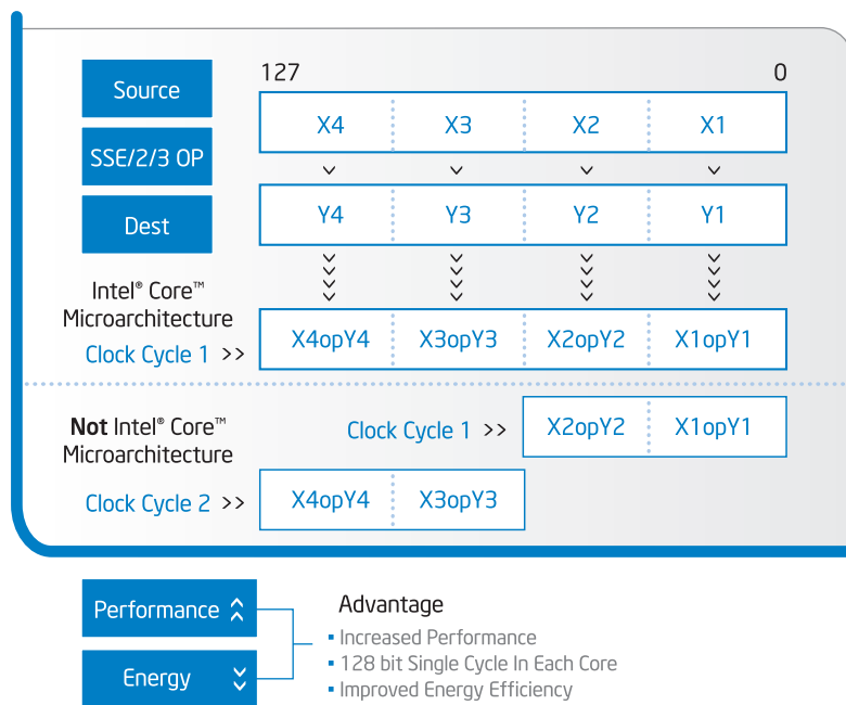
Intel® Advanced Digital Media Boost SSE Operation (SSE/SSE2/SSE3)
