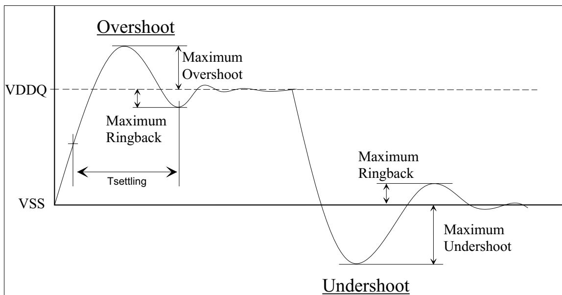
Figure 5-2 Overshoot & Undershoot
