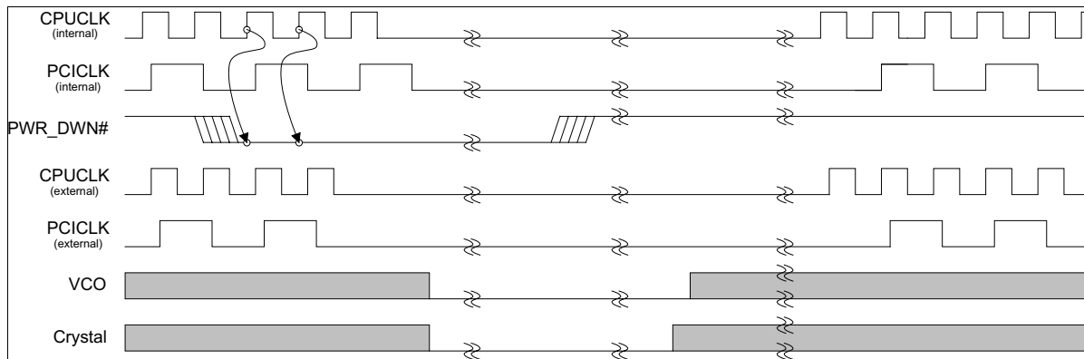
Figure 8-6 CK100 PWR_DWN# Timing Diagram
