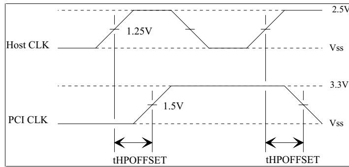
Figure 3-2 Host CLK to PCI CLK Offset
