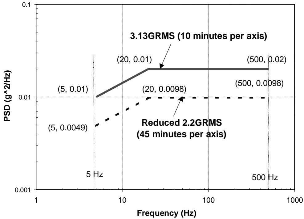
Figure 7. Power spectral density ( PSD) curve for vibration tests.
