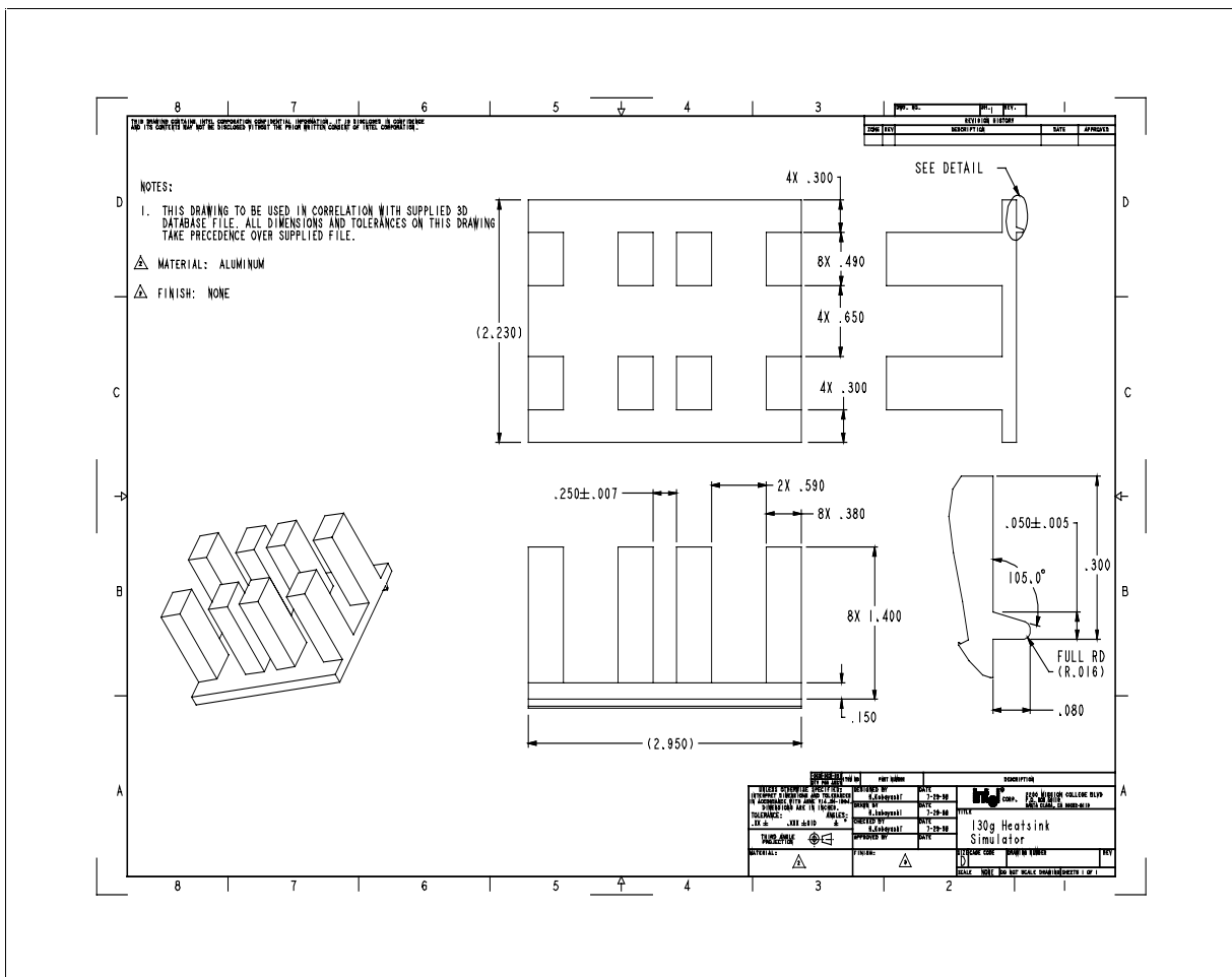
Figure 4. Schematic of heat sink simulator for mechanical shock and vibration tests.
