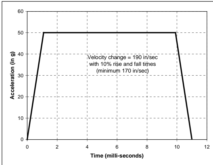
Figure 9. Trapezoidal shock wave form for the board level mechanical shock test.
