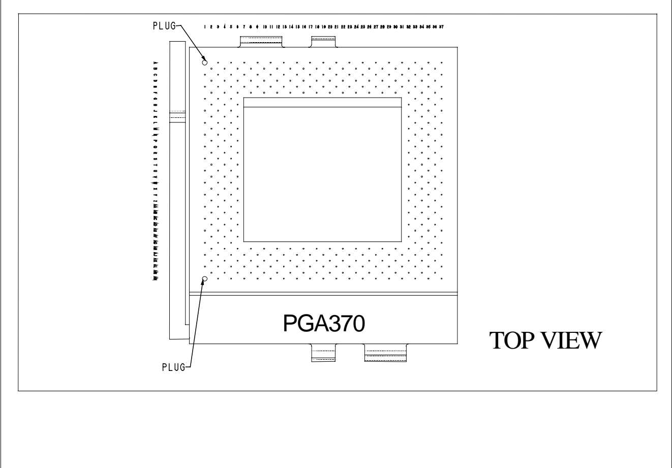
Figure 1. Schematic of the 370-pin socket
