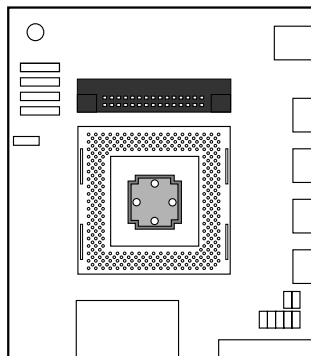
Typical LIF socket (no handle)
