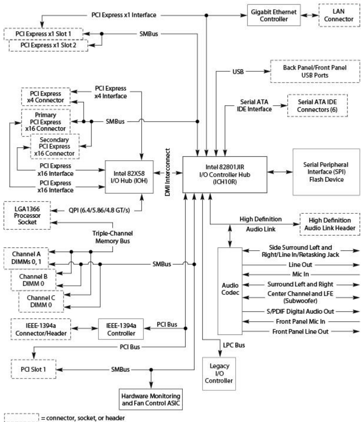
Figure 2. Block Diagram
