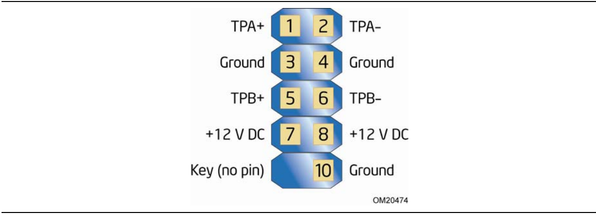
Figure 13. Connection Diagram for IEEE 1394a Header
