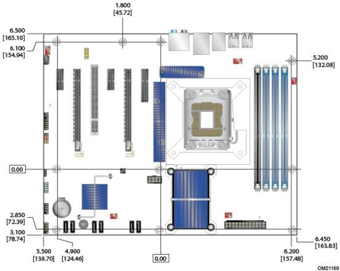
Figure 15. Board Dimensions
