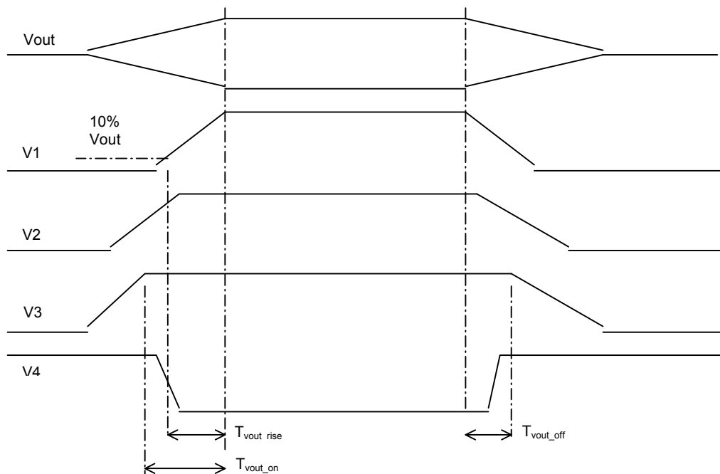
Figure 13. Output Voltage Timing
