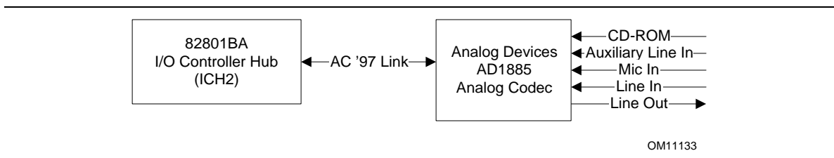
Figure 4. Block Diagram of Audio Subsystem
