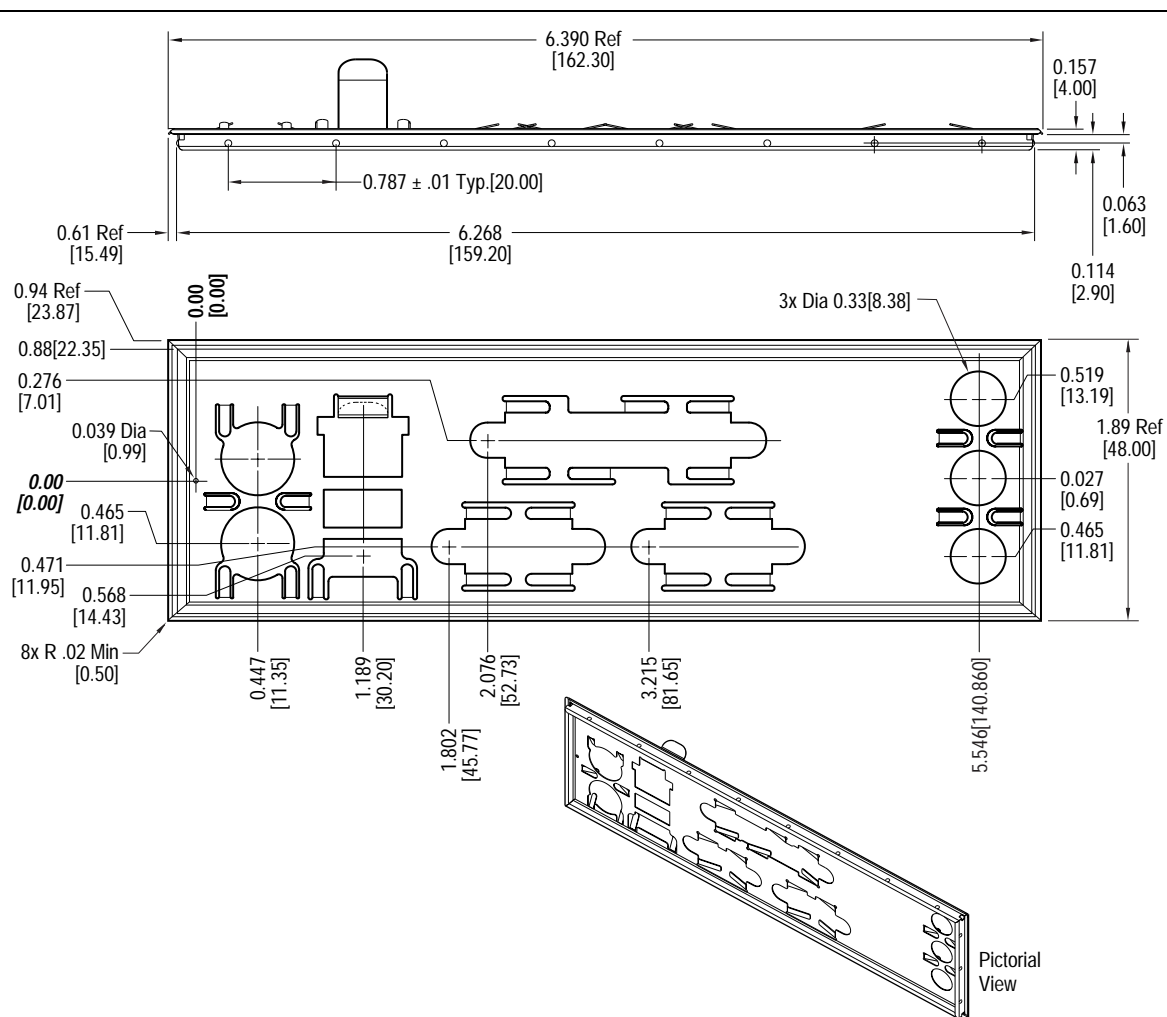
Figure 14. Back Panel I/O Shield Dimensions
