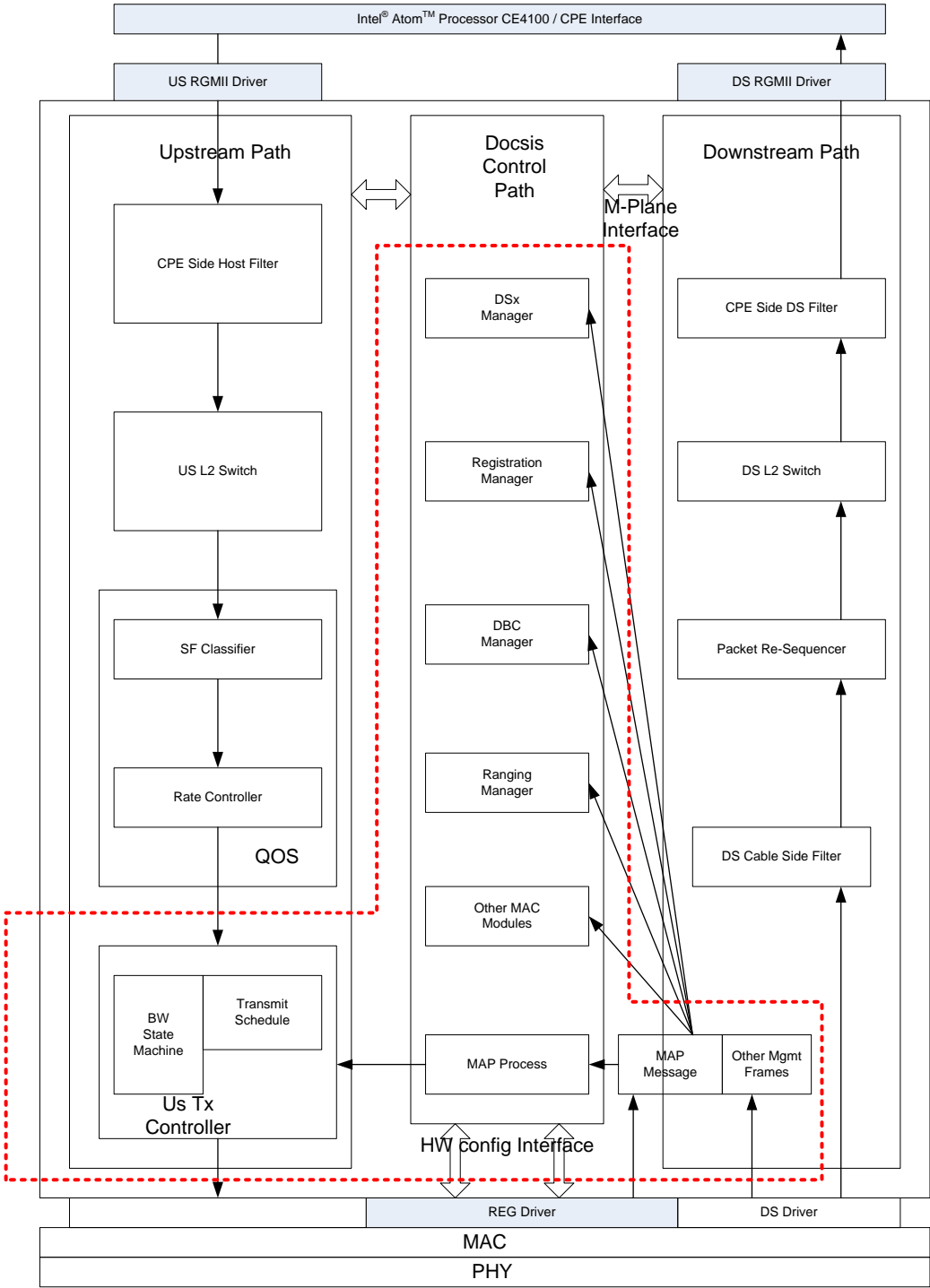
Figure 9 Practical Design Split of Functionality across Processors, on the Basis of Control and Data Processing
