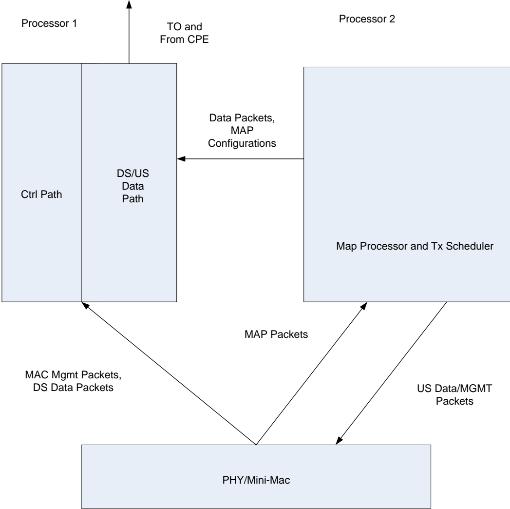
Figure 10 Conceptual Design MAP-Processor/TX-Scheduler on a Separate Processor, with OS
