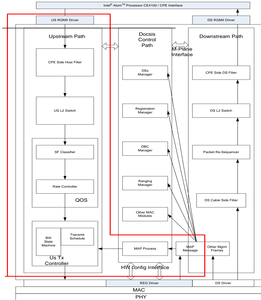
Figure 5 Practical Design
