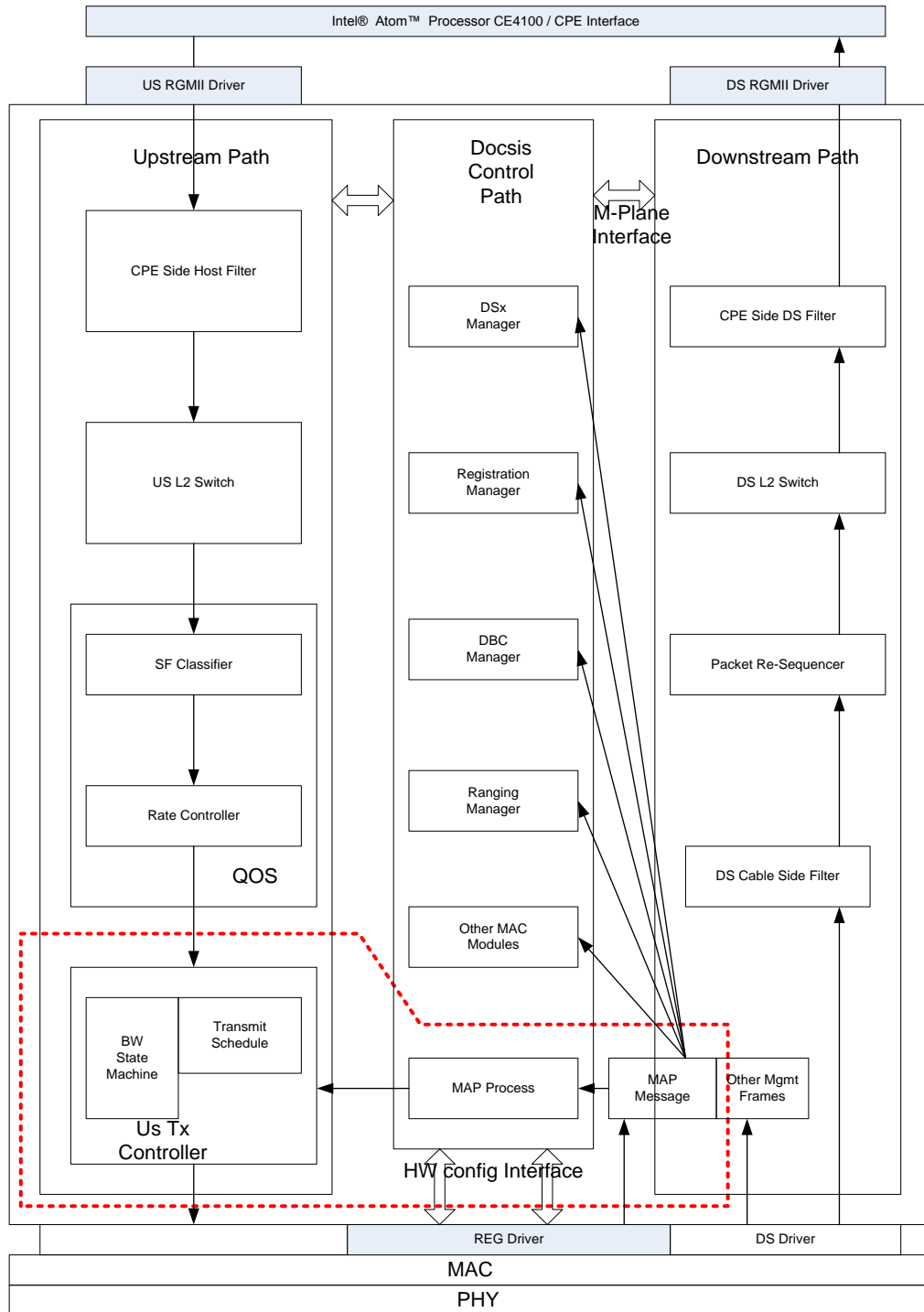
Figure 13 Practical Design MAP-Processor/TX-Scheduler on a separate processor, without OS
