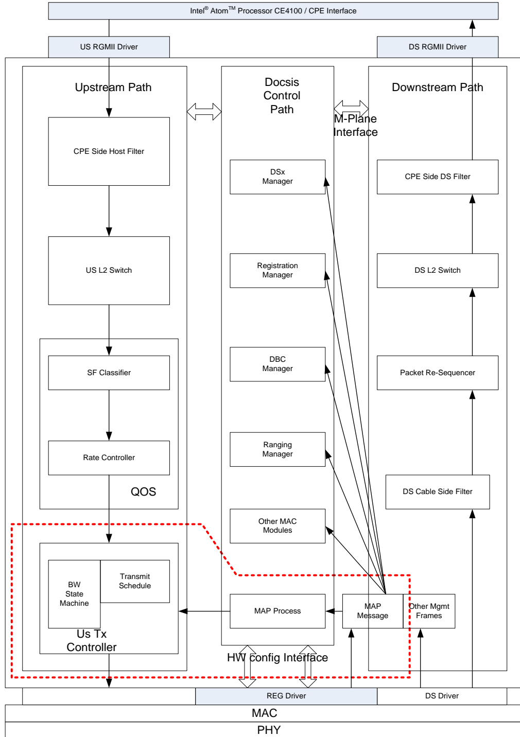
Figure 11 Practical Design MAP-Processor/TX-Scheduler on a Separate Processor, with OS
