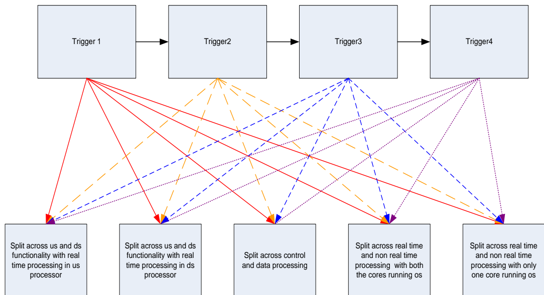
Figure 3 Relationship Between Triggers and Suggested MultiProcessor Solution
