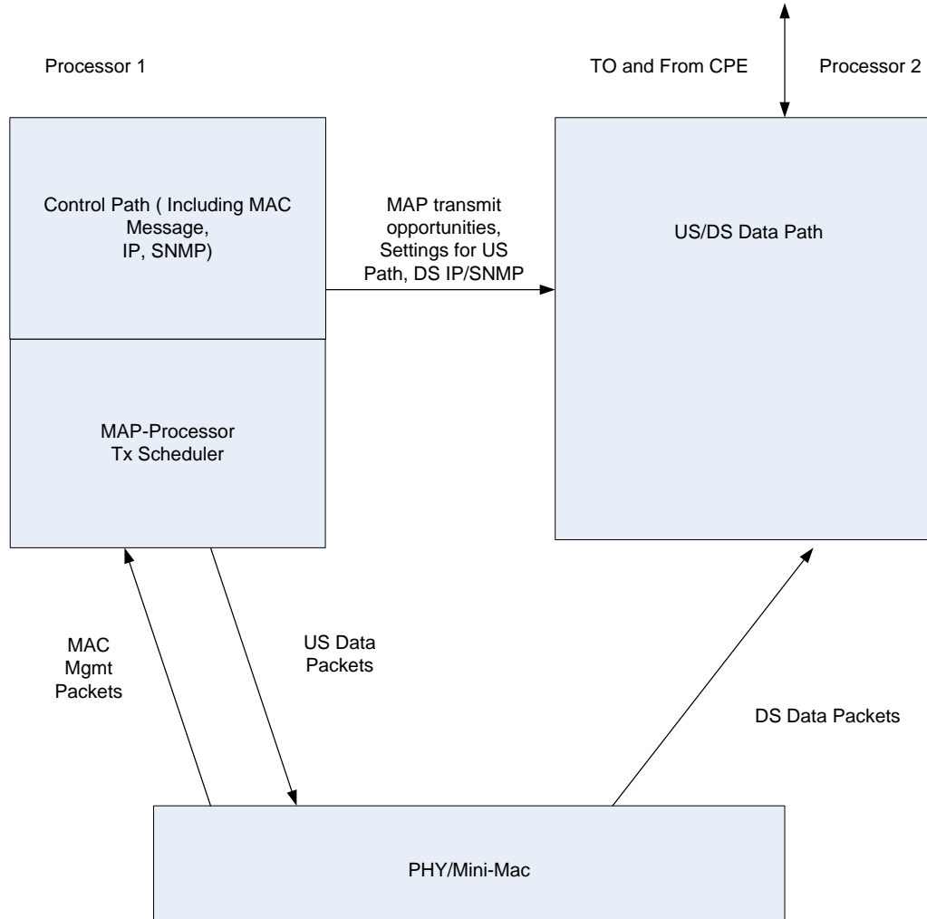
Figure 8 Conceptual Design Split of Functionality across Processors, on the Basis of Control and Data Processing
