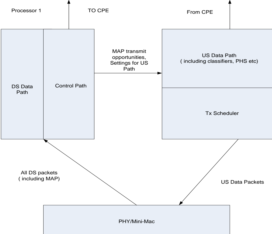
Figure 6 Conceptual Design of Split of Functionality across Processors, on the Basis of Non Time Critical US/DS Functionality
