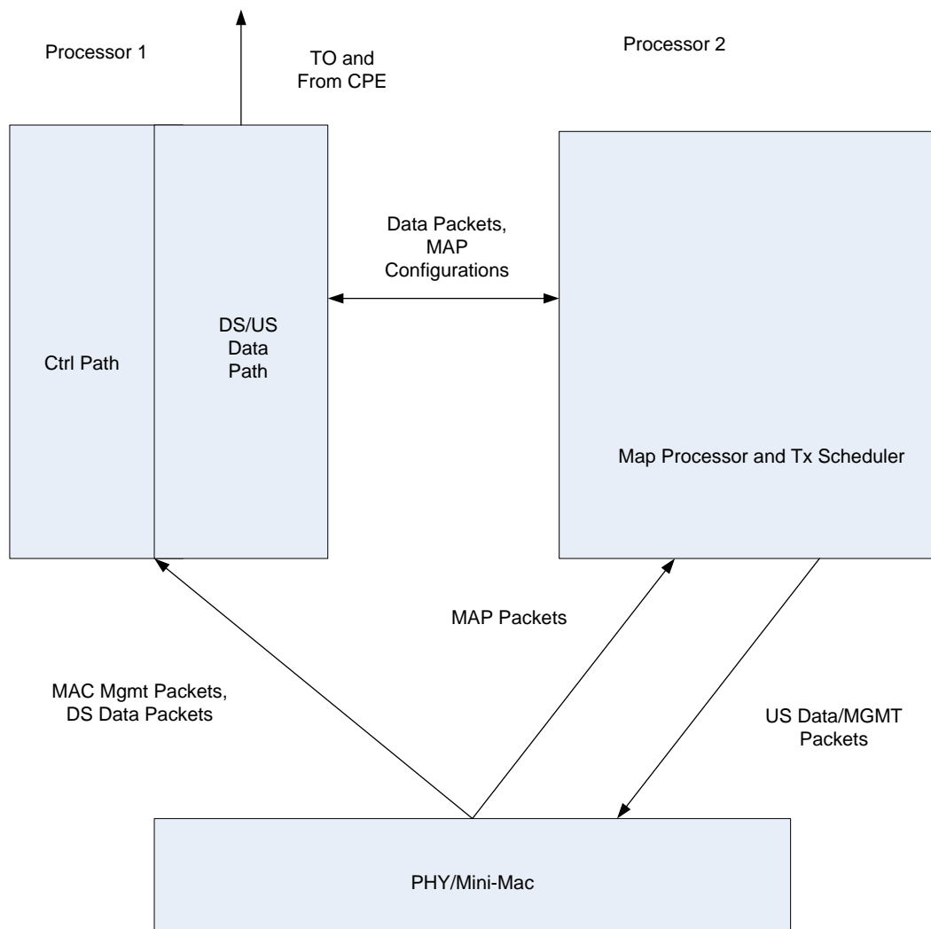
Figure 12 Conceptual Design MAP-Processor/TX-Scheduler on a separate processor, without OS
