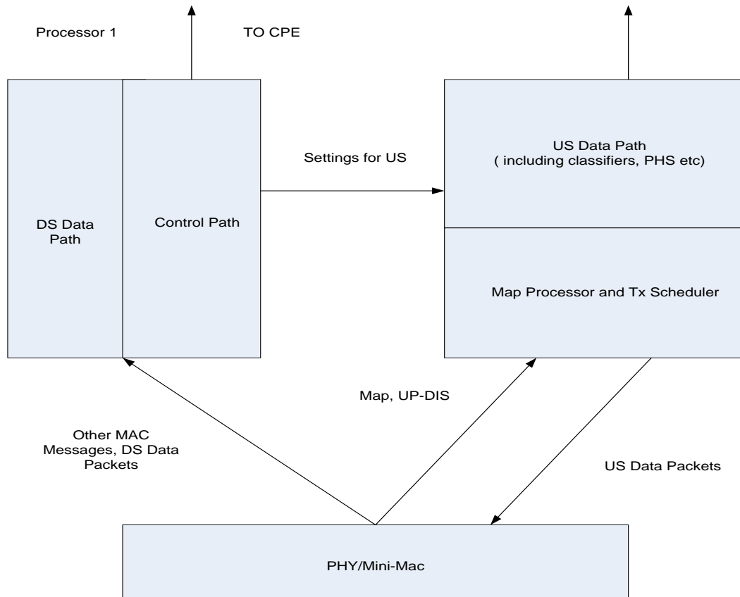
Figure 4 Conceptual Design
