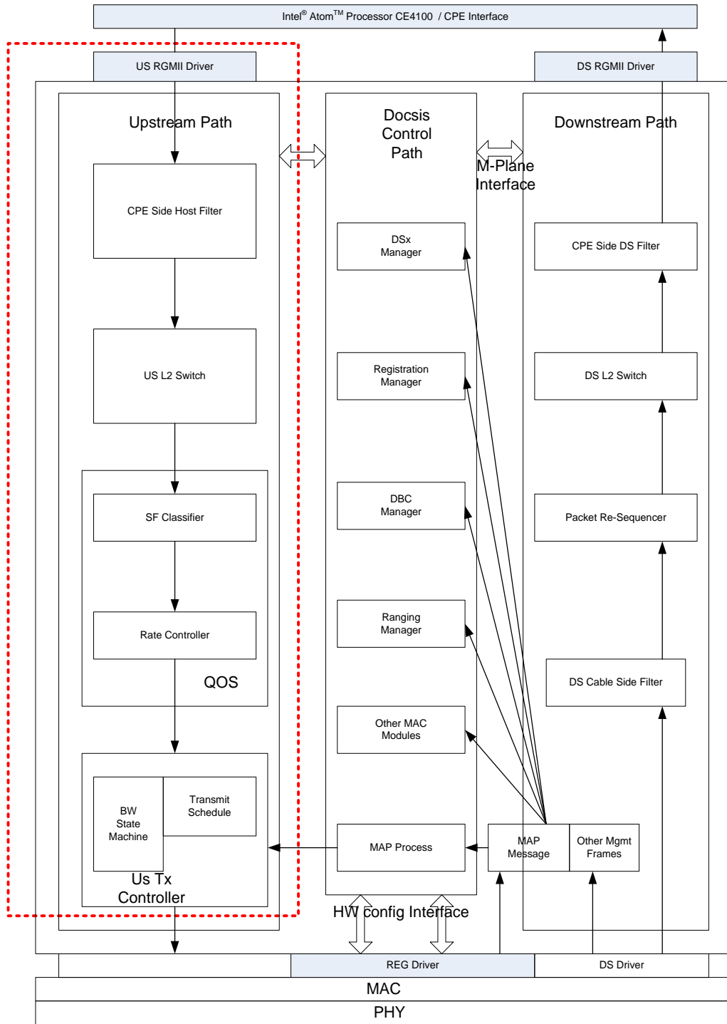
Figure 7 Practical Design of Split of Functionality across Processors, on the Basis of Non Time Critical US/DS Functionality
