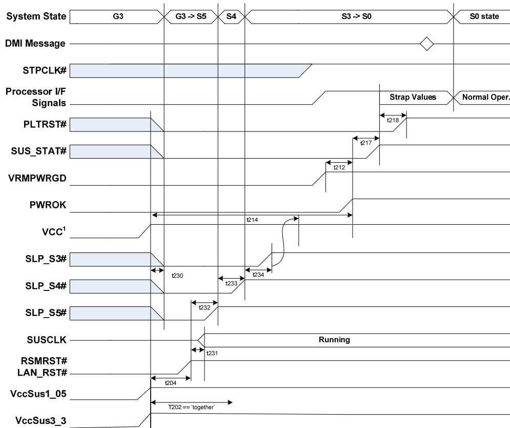
Figure 5. G3 (Mechanical Off) to S0 Timings - Combined
