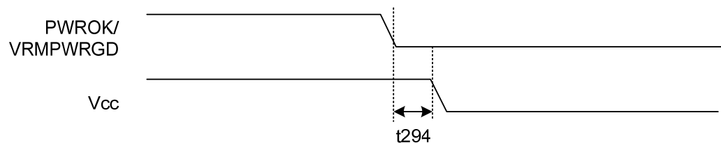
Figure 6. S0 to G3 Timings (Desktop Only) – Normal Operation
