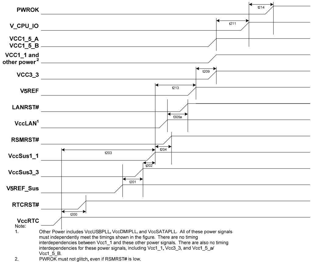
Figure 2. Power Sequencing and Reset Signal Timings - Normal
