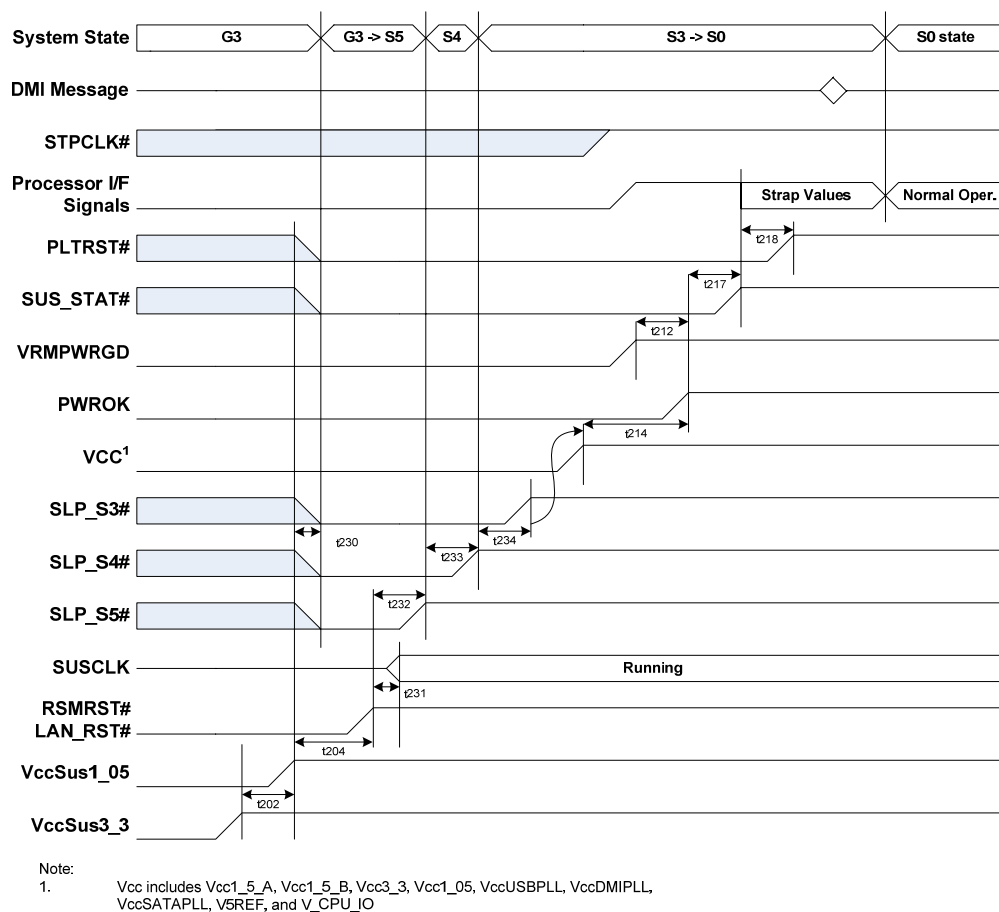
Figure 4. G3 (Mechanical Off) to S0 Timings - Normal
