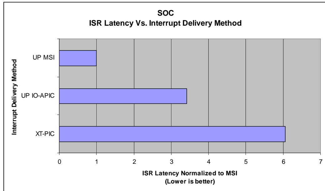
Figure 10. Normalized UP SoC Results
