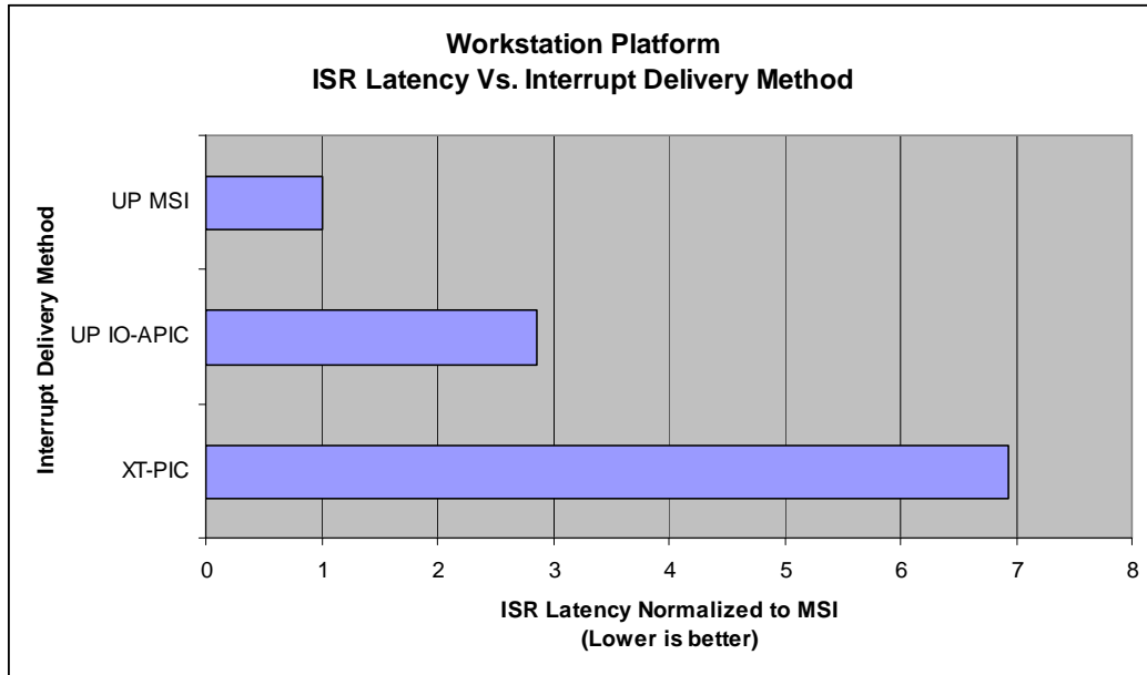
Figure 9. Normalized UP Workstation Results
