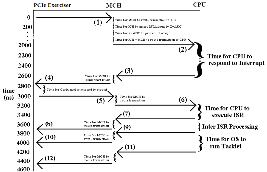
Figure 8. PCIe* Analyzer Trace of Legacy (XT-PIC/IO-APIC) Events
