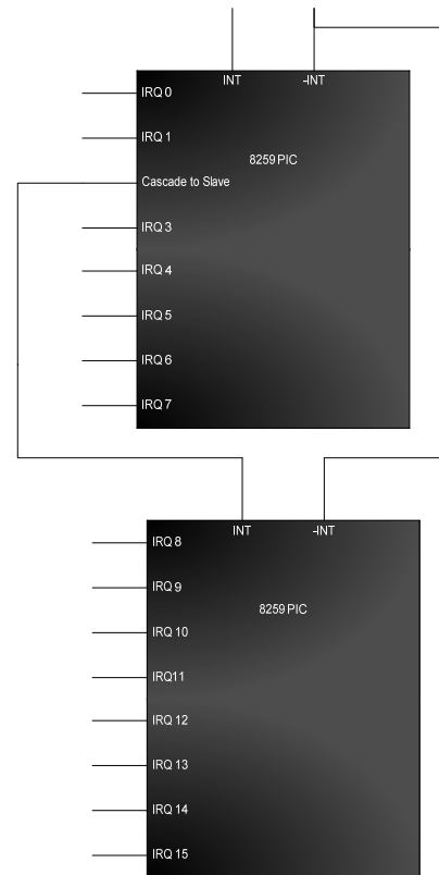
Figure 2. XT-PIC Cascade
