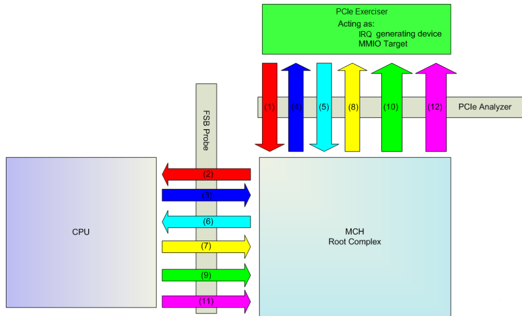
Figure 6. PCIe* Visible Legacy (XT-PIC/IO-APIC) Events
