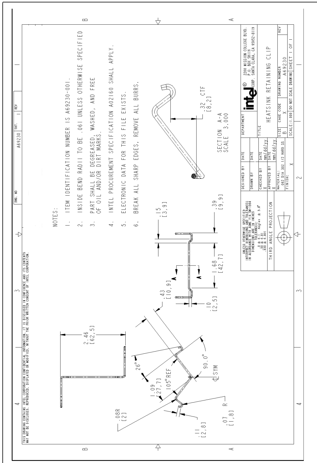
Figure 13. Torsional Clip
