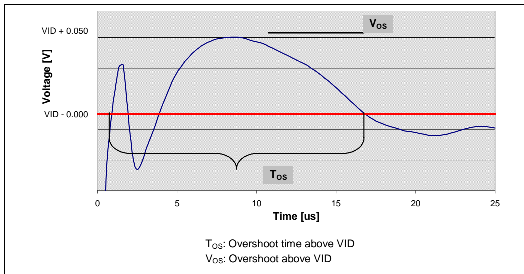
Figure 4. V CC Overshoot Example Waveform
