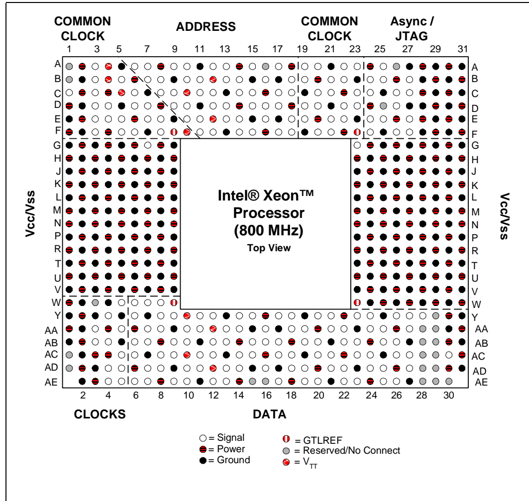
Figure 10. Processor Pinout Coordinates, Top View
