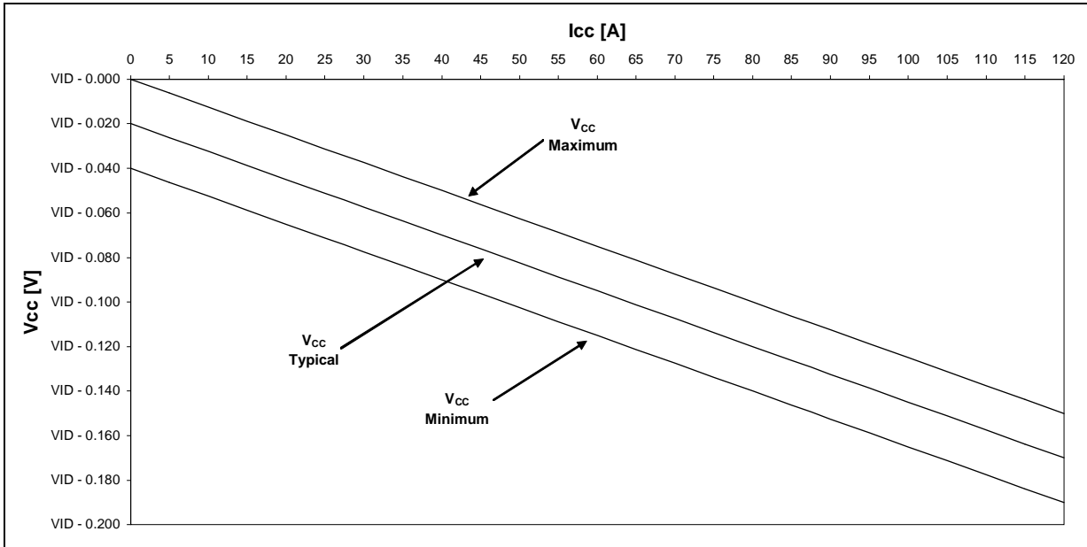
Figure 3. V CC Static and Transient Tolerance
