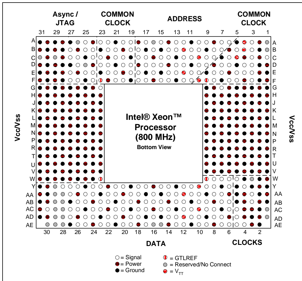
Figure 11. Processor Pinout Coordinates, Bottom View
