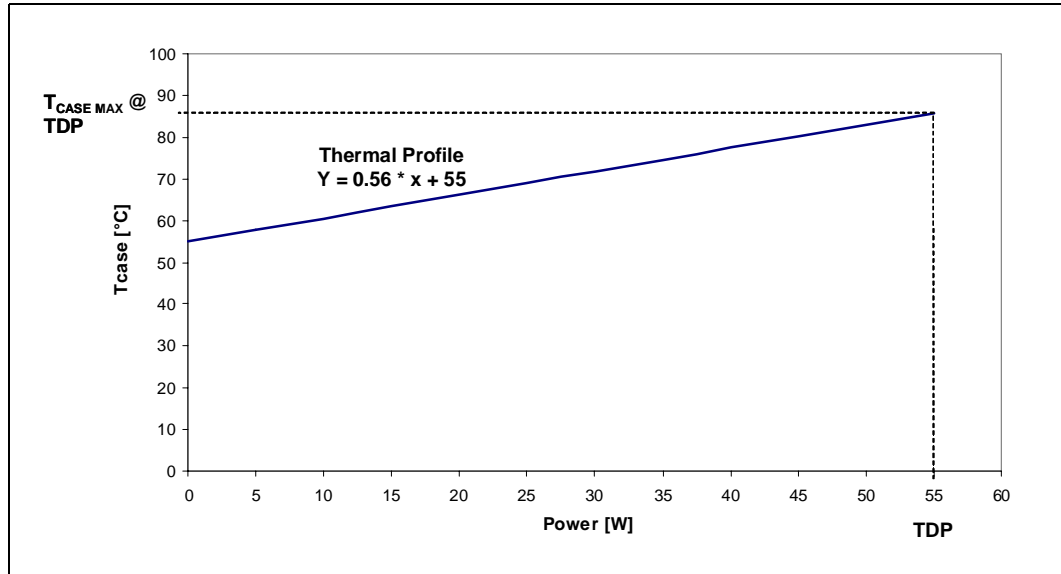
Figure 12. Low Voltage Intel® Xeon™ Processor with 800 MHz System Bus Thermal Profile
