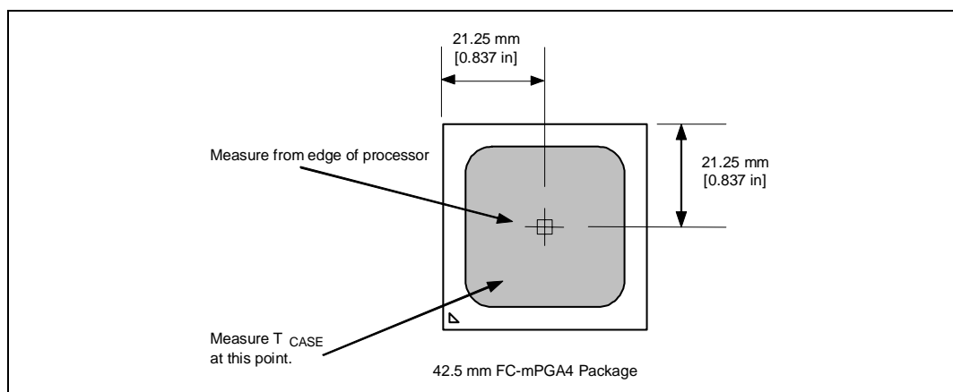
Figure 13. Case Temperature ( T_{CASE} ) Measurement Location
