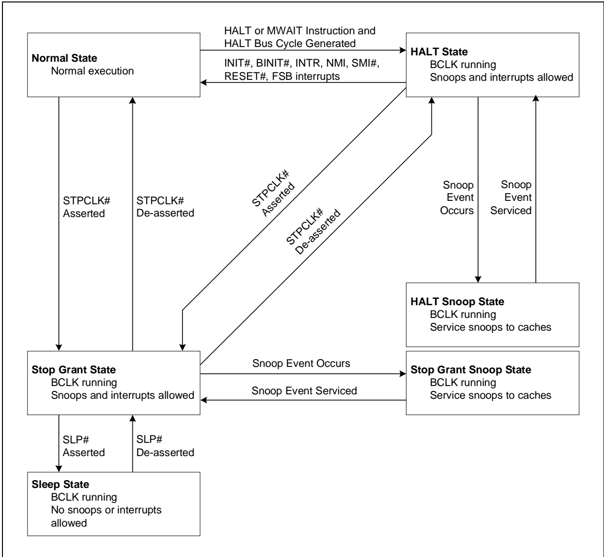
Figure 14. Stop Clock State Machine
