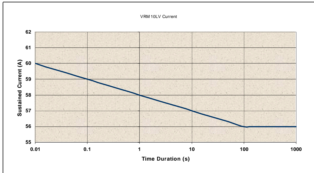
Figure 2. Low Voltage Intel® Xeon™ Processor with 800 MHz System Bus Load Current vs. Time (VRM 10.0)
